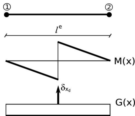
Figure 4 Interpolation functions for the discontinuity
