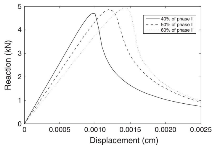
Figure 5 Macroscopic responses for the 2D uniaxial tension test with three different specimens
